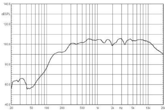
Freq. Response (dB SPL, 1W,1m)
