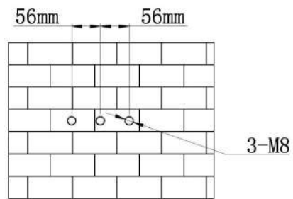
Positioning Dimensions & Diagram
