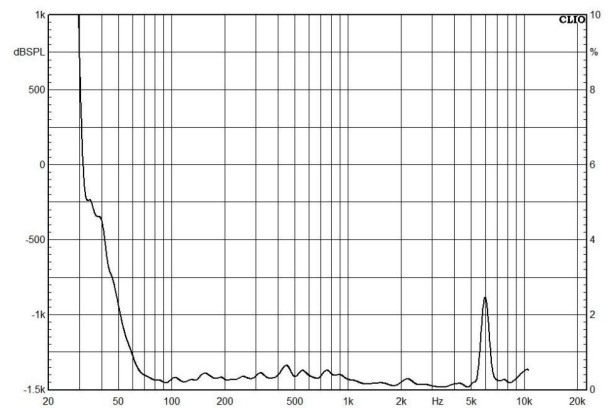
Distortion Characteristic (THD< 1.5%, 1W, 1m, 100Hz-10kHz)
